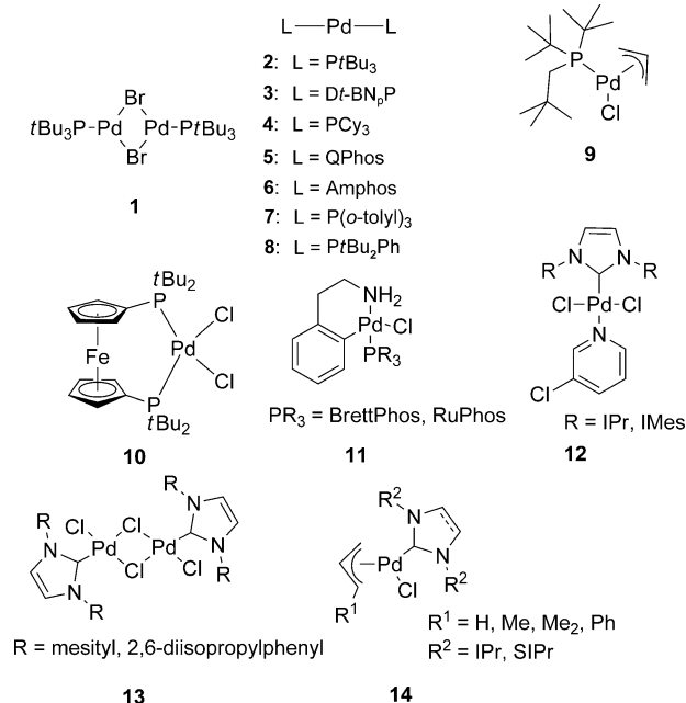
Scheme 26. Selected preformed palladium catalysts for various cross-coupling reactions. [147–150, 153–159] Amphos = \text{PtBu}_2\text{C}_6\text{H}_4\text{NMe}_2 ; Dt-BNp = di( tert -butyl)neopentylphosphine.
