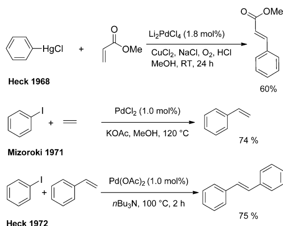
Scheme 11. The first palladium(II)-catalyzed coupling reactions. [53,55,56]
