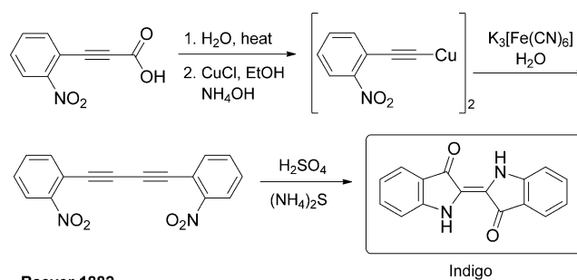
Scheme 4. Baeyer's synthesis of indigo. [13]
