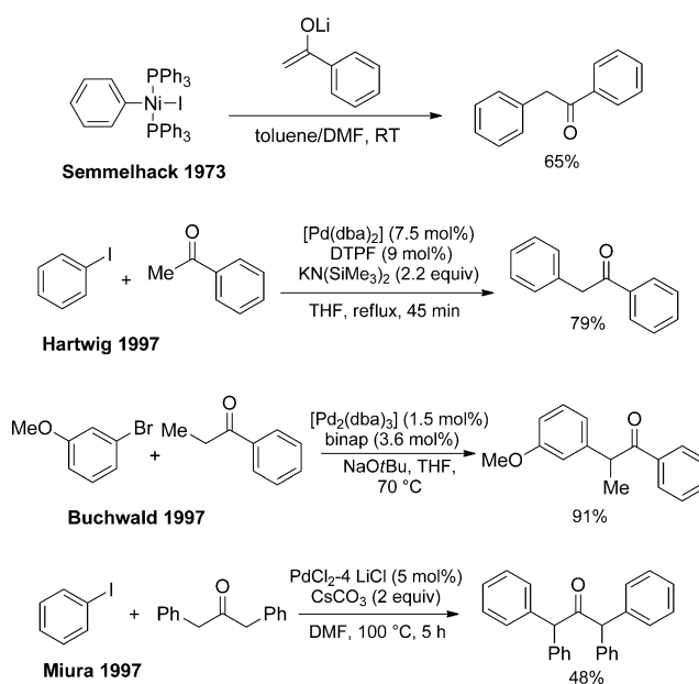
Scheme 30. History of the \alpha -arylation reaction. [167–170] DTPF = 1,1'-bis(di- o -tolylphosphino)ferrocene.
