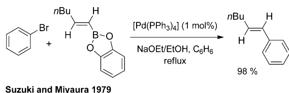
Scheme 17. The Suzuki–Miyaura cross-coupling reaction. [89]
