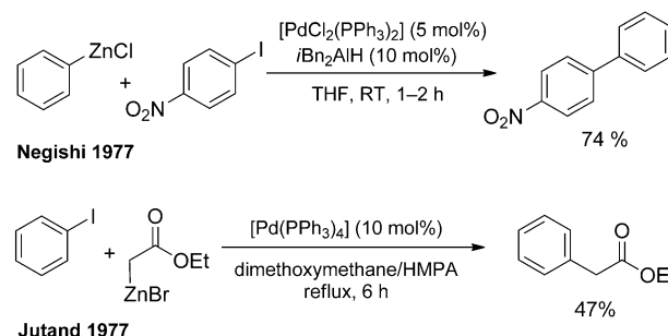
Scheme 15. The Negishi cross-coupling reaction. [76–78]
